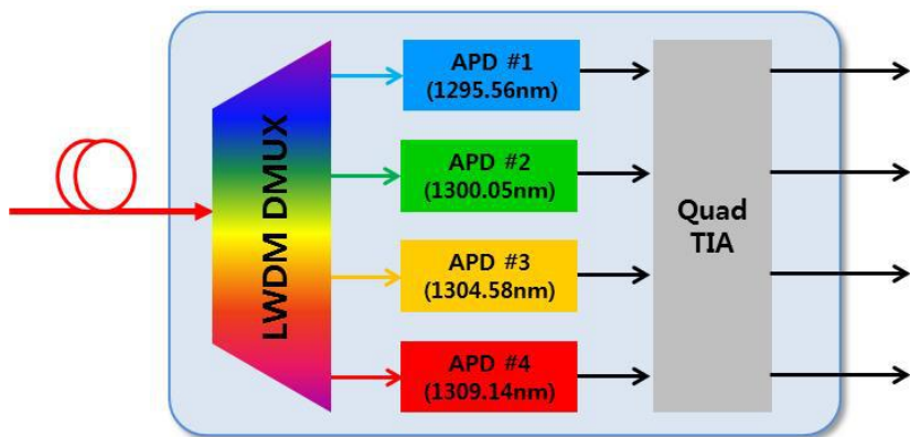
Block Diagram
